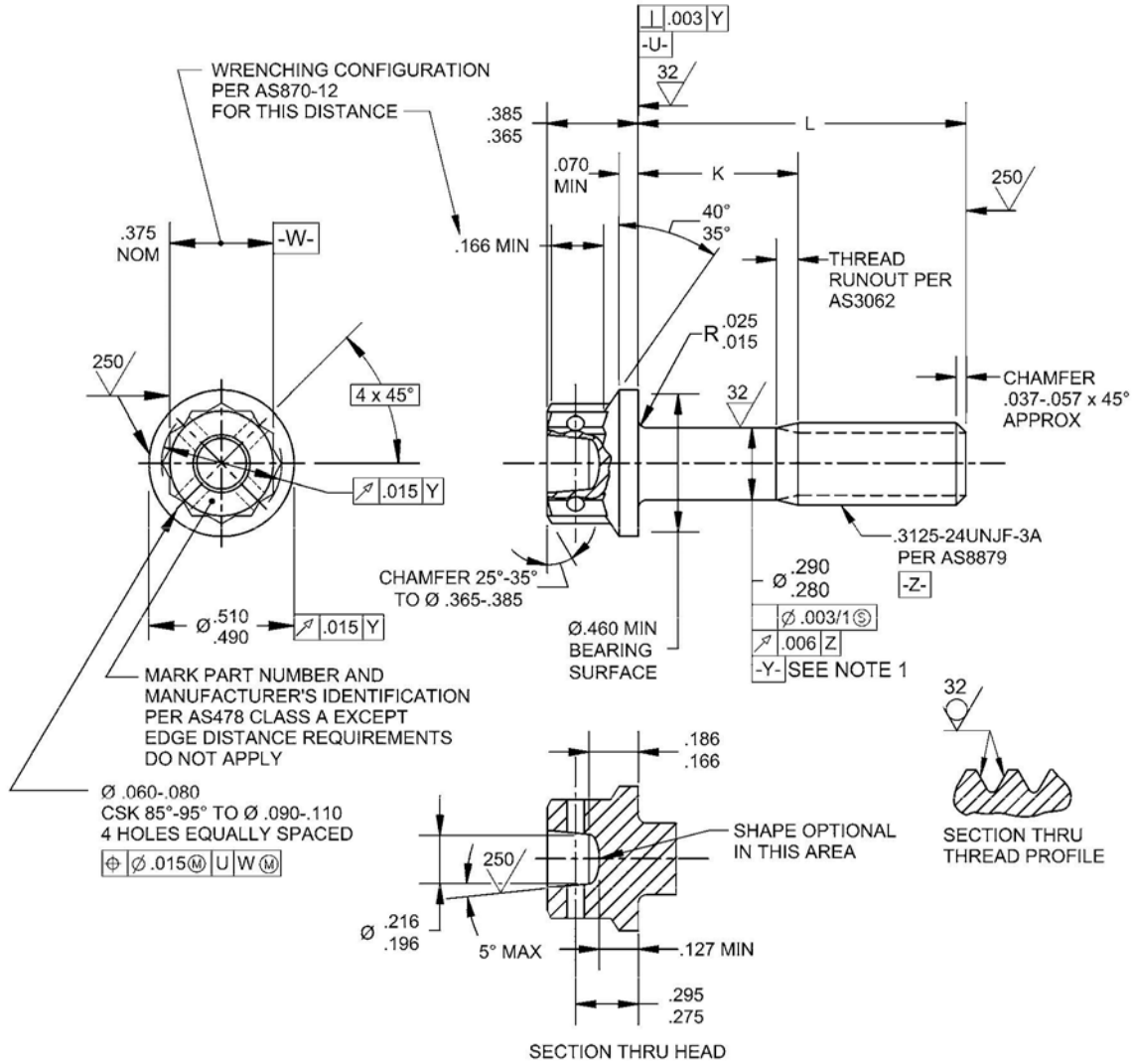
FIGURE 1 - BOLT
